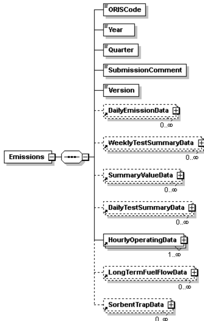
Figure 2: Emissions XML Elements
