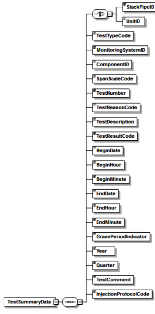
Figure 51: Miscellaneous Tests XML Structure
