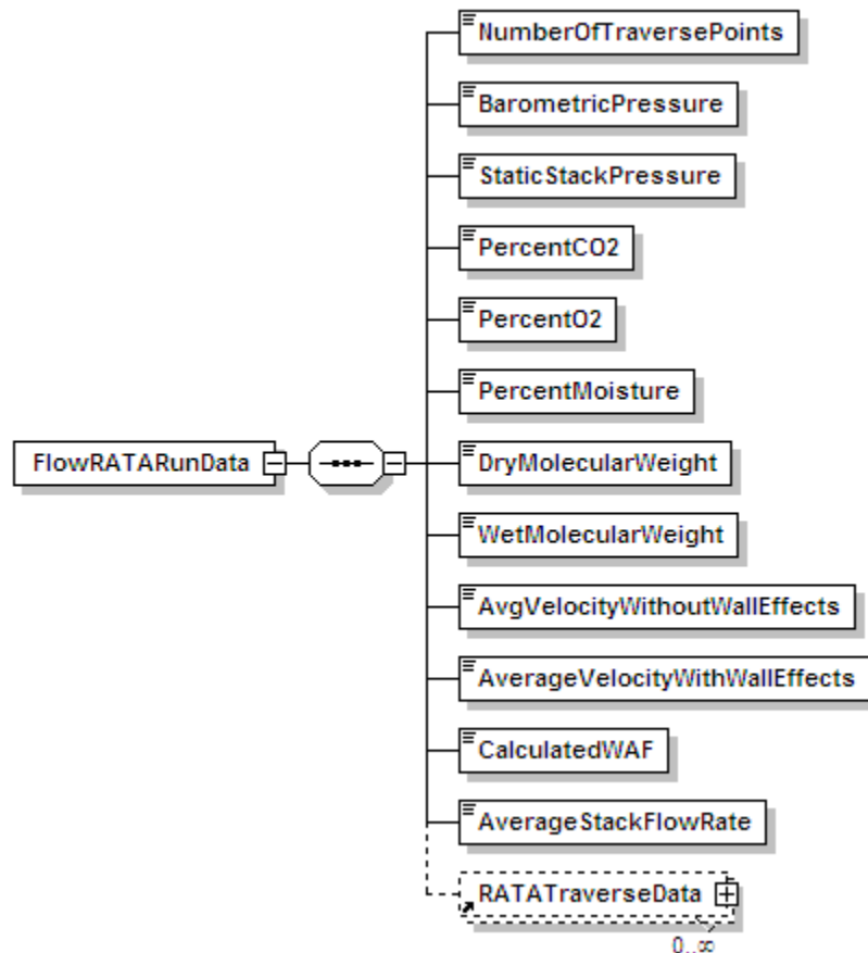
Figure 20: Flow RATA Run Data XML Elements
