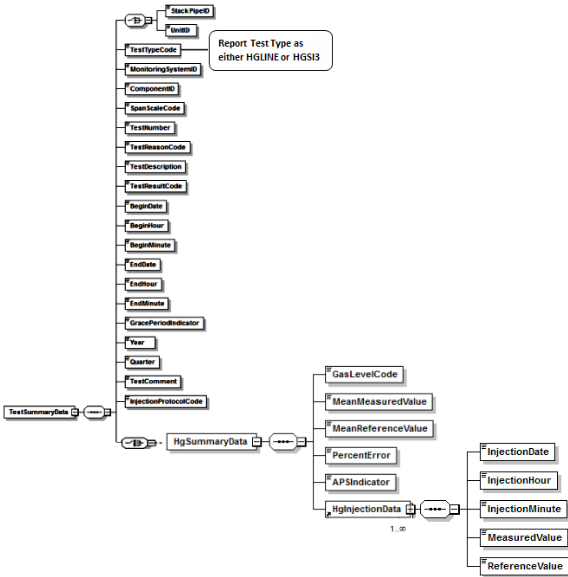
Figure 13: Hg Linearity/System Integrity Check XML Elements
