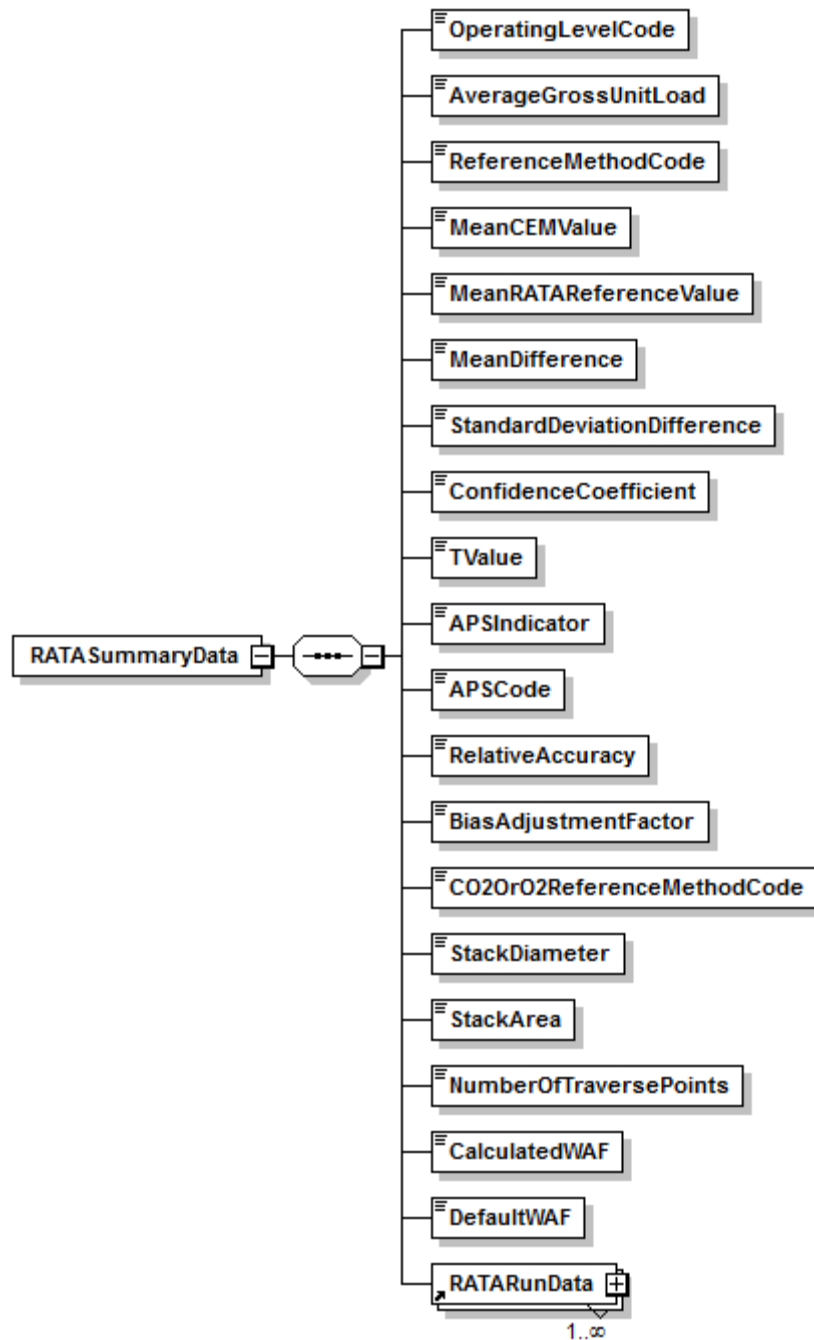
Figure 18: RATA Summary Data XML Elements
