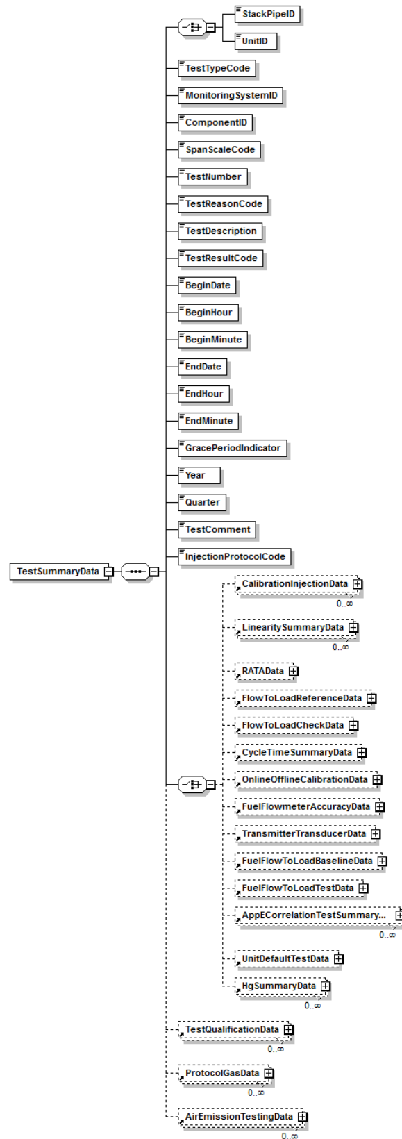
Figure 3: Test Summary Data XML Elements
