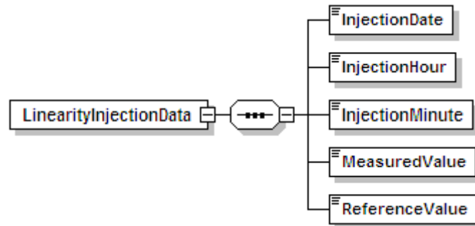
Figure 11: Linearity Injection Data XML Elements
